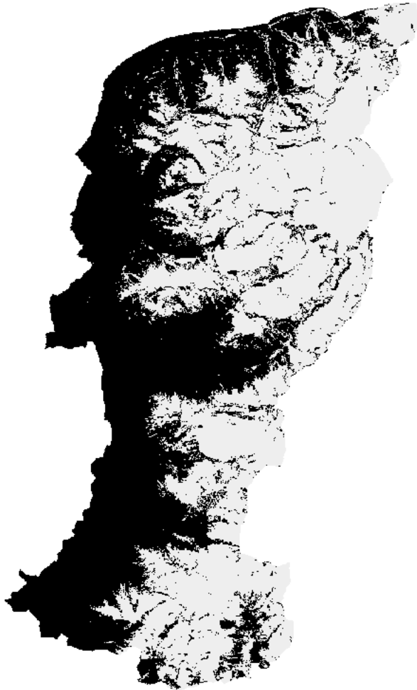
Snow mask
